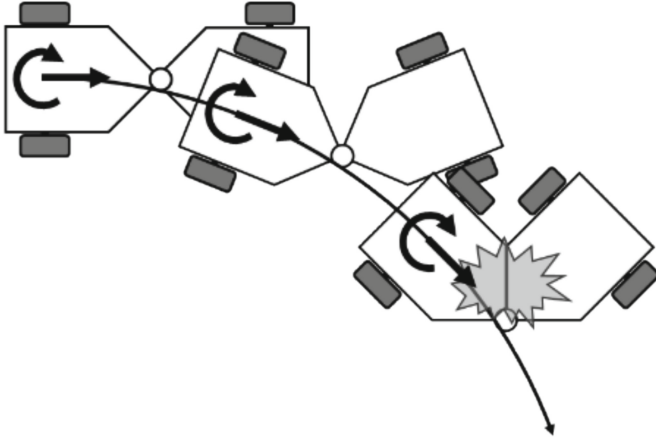
Fig. 2. Jackknifing.
